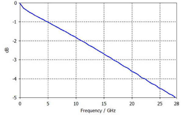
Insertion loss OSFP HCB ML4064-HCB
